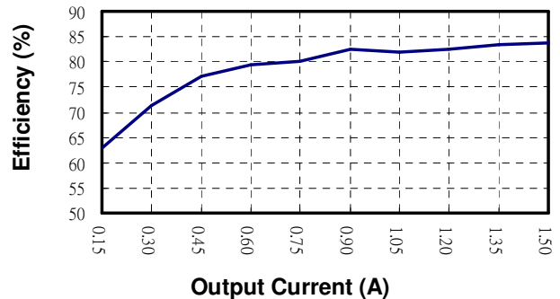
BOB8-48S1H3 Output Current vs. Efficiency
