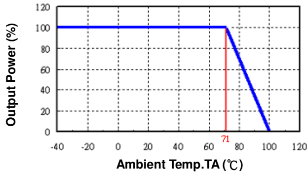
BOB8H3 Series Power Derating Curve(5)
