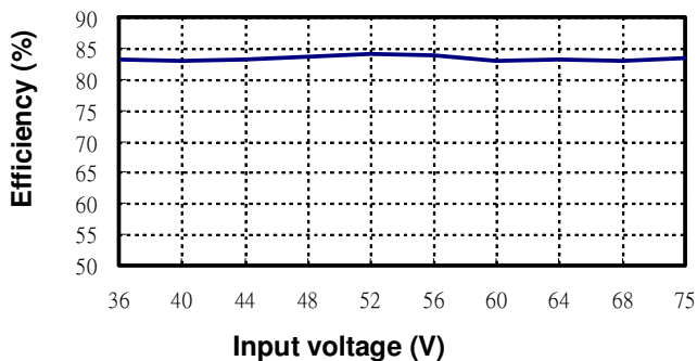
BOB8-48S1H3 Input voltage vs. Efficiency
