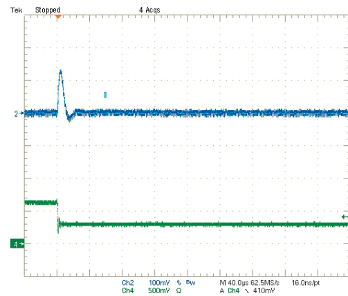
Step Load Transient Response (Vin=5V, Vout=1.2V, Cload=0, Iout=3A to 1.5A) Trace 2=Vout, 100 mV/div. Trace 4=Iout, 2.5A/div.
