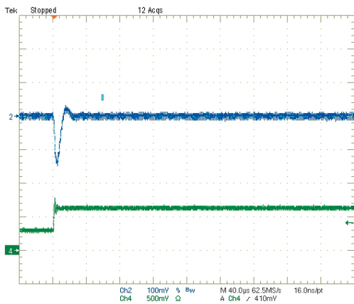
Step Load Transient Response (Vin=5V, Vout=1.2V, Cload=0, Iout=1.5A to 3A) Trace 2=Vout, 100 mV/div. Trace 4=Iout, 2.5A/div.
