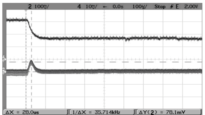
Step Load Transient Response (Vin=12V, Vout=2.5V, Cloud=0, Iout=6A to 3A) Trace 2=Vout, 100 mV/div. Trace 4=Iout, 2A/div.
