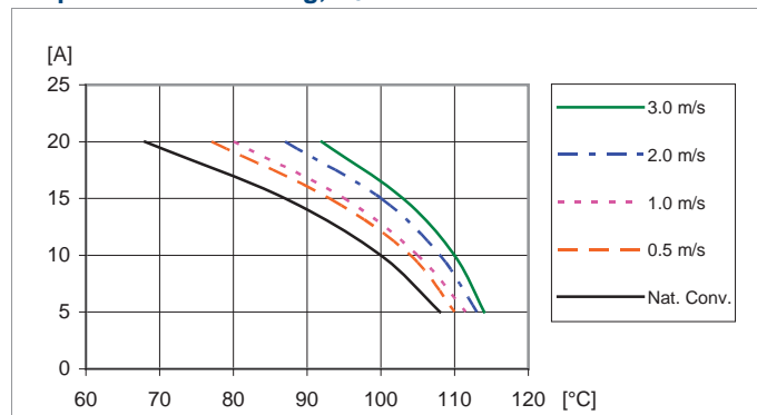
Output Current Derating, V_O = 1.8\text{ V}
