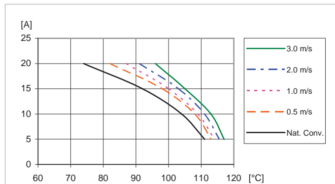
Output Current Derating, V_O = 0.6\text{ V}
