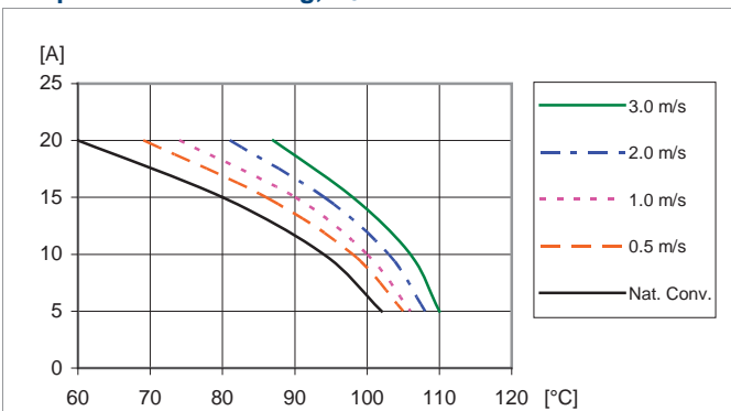
Output Current Derating, V_O = 3.3\text{ V}
