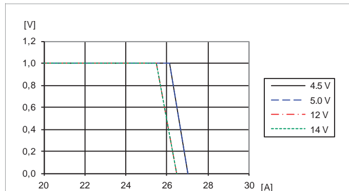
Current Limit Characteristics, V_O = 1.0\text{ V}
